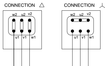
SINGLE SPEED
